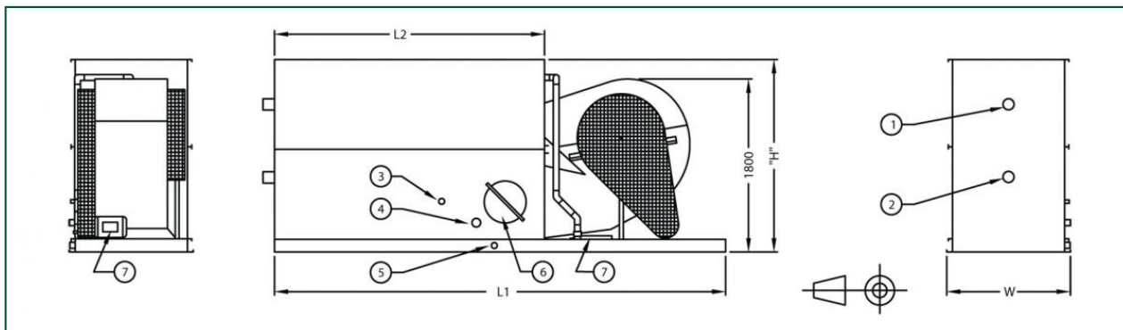
1. Refrigerant in ND100; 2. Refrigerant out ND100; 3. Make up ND25; 4. Overflow ND50 on VCL 042-119 & 133 - ND80 on VCL 131 & 140-159; 5. Drain ND50; 6. Access; 7. Spray pump; 8. Fan motor.
