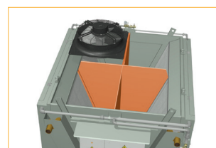
Internal partitioning panels* for individual air intake
