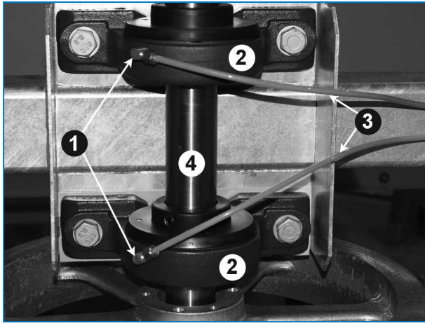
Location of fan shaft bearings and lube fittings
