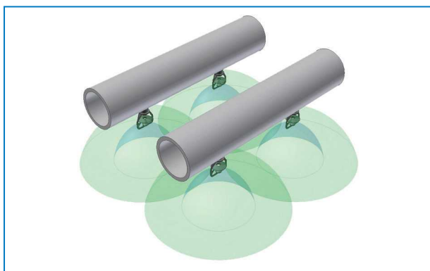
Nozzle spray distribution type for closed circuit cooling tower
